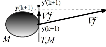
Fig. 1: Illustration of an optimization iterate
