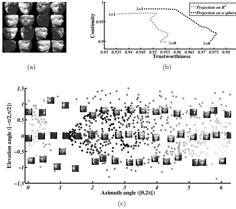
Fig. 2: (a) Sample of face data base; (b) comparison between the projections on \mathbb{R}^2 and on the sphere with the trustworthiness and the continuity measure; (c) Representation of the projected face data on the sphere for \lambda = 0.7 in the spherical coordinate space (the color varies as the azimuthal angle of the camera does). Only a few data are represented as faces to increase the readability of the figure and to show the smoothness of the projection.
